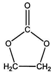
Ethylene Carbonate (EC)
